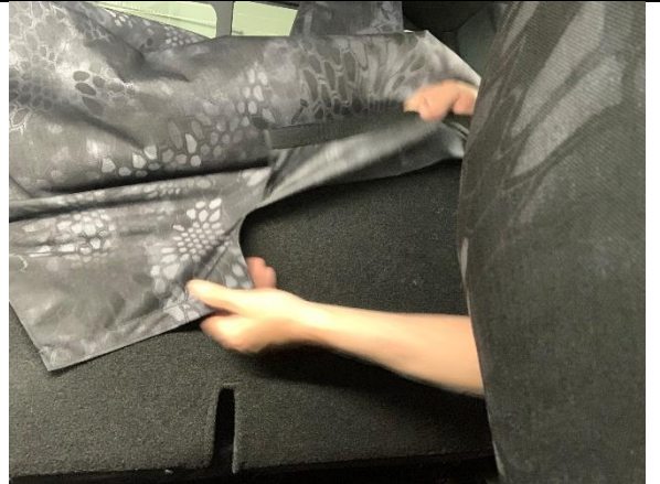
Step 16. Driver Bottom/DB: Lift the seat bottoms up and slide the cover on with the extending Hook Velcro™ to the top side, and the 1" Hook Velcro™ sewn inside to the underside.
